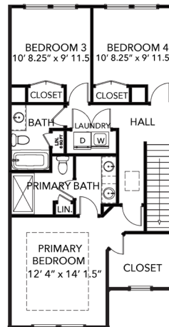
THIRD FLOOR
